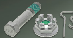
COATED FASTENERS Repel-TEK™ Coated Fasteners Hardware is coated with heavy-duty anti-corrosion coating. This prevents future repair frustration- common when pinch bolts seize to the steering knuckle.
