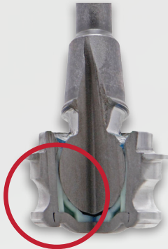
OEM BALL JOINT Plastic bearing with sealed design
