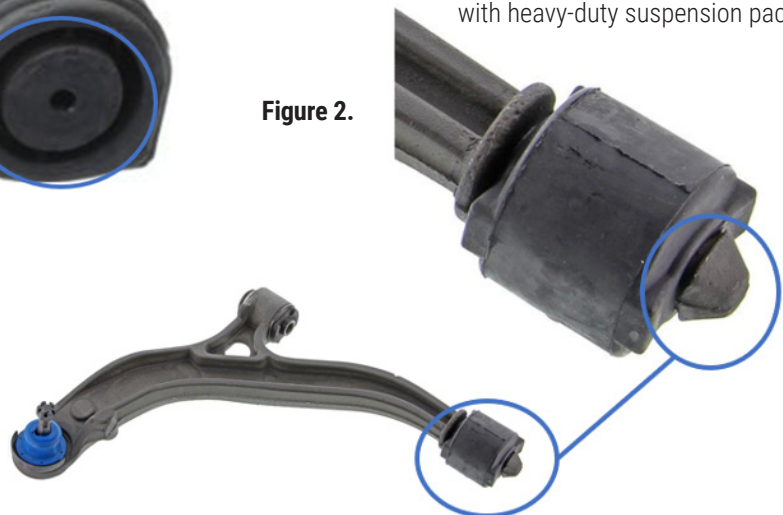
Figure 2. Compliance bushing mount with tabbed end (circled) for vehicles with heavy-duty suspension package
