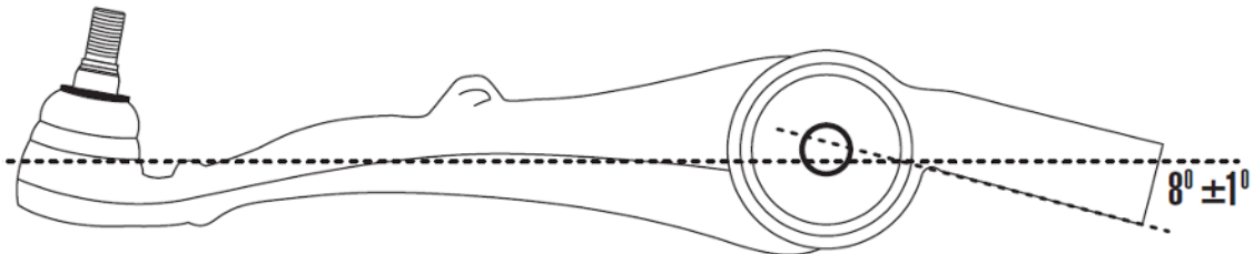
Figure 2. Correct installation orientation is achieved when center line of control arm and under edge of bracket are aligned within 8° (±1°).
