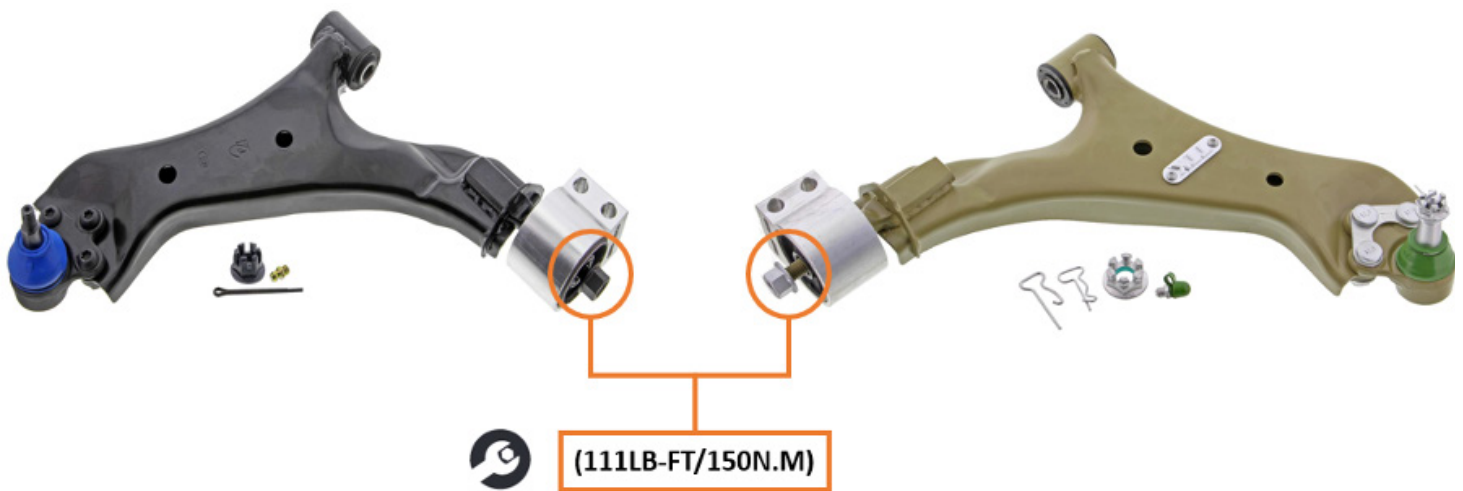
Figure 1. Bushing bracket nut (circled above) must be correctly torqued after fitting control arm to vehicle
