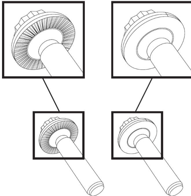
Figure 1. 12-point bolt with ribbing underneath bolt head (left) and 12-point bolt without ribbing (right)
