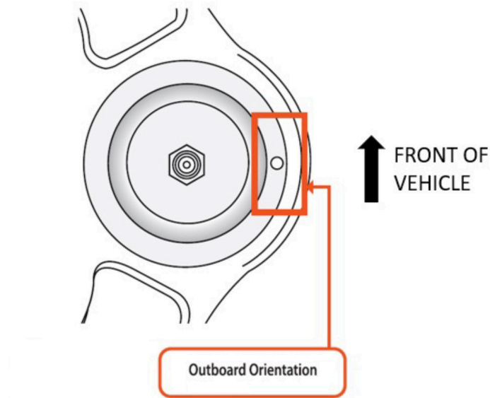
Figure 3. Correct ball joint installation orientation when mated to front upper control arm. Note drilled index mark position (highlighted orange box)
