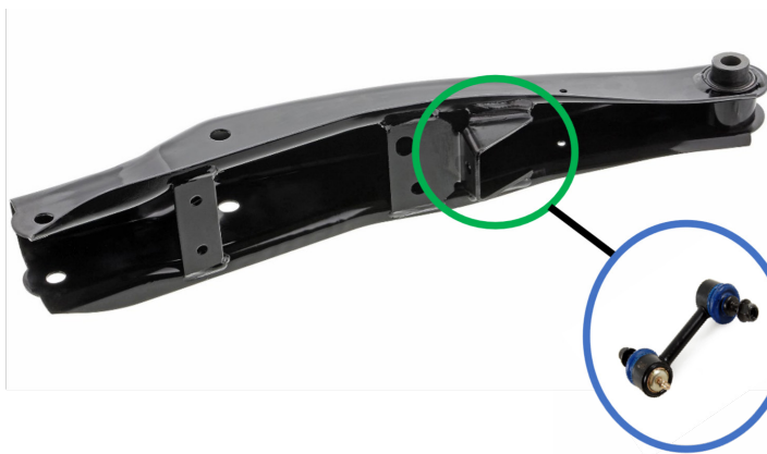
Figure 1. Inboard mount location on CMS501232 for style 1 stabilizer link
