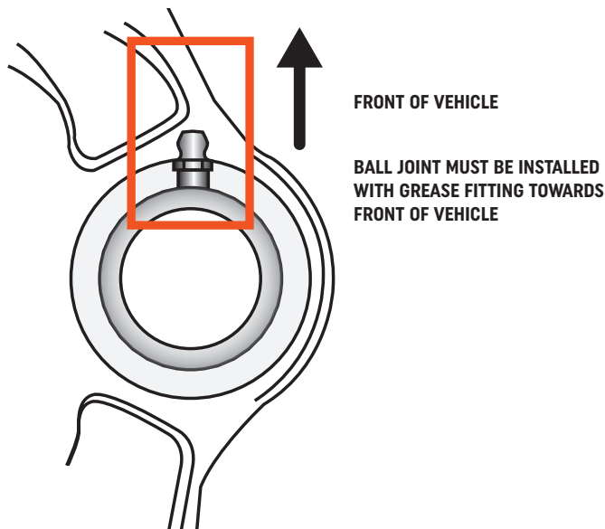
Figure 1: Correct Ball Joint Installation Orientation
