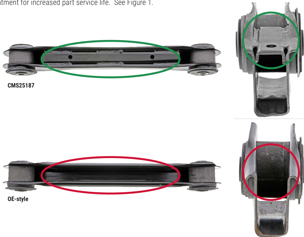
Figure 1. Mevotech Supreme control arm with improved stamping profile featuring bracing (top) vs OE-style control arm (bottom)
