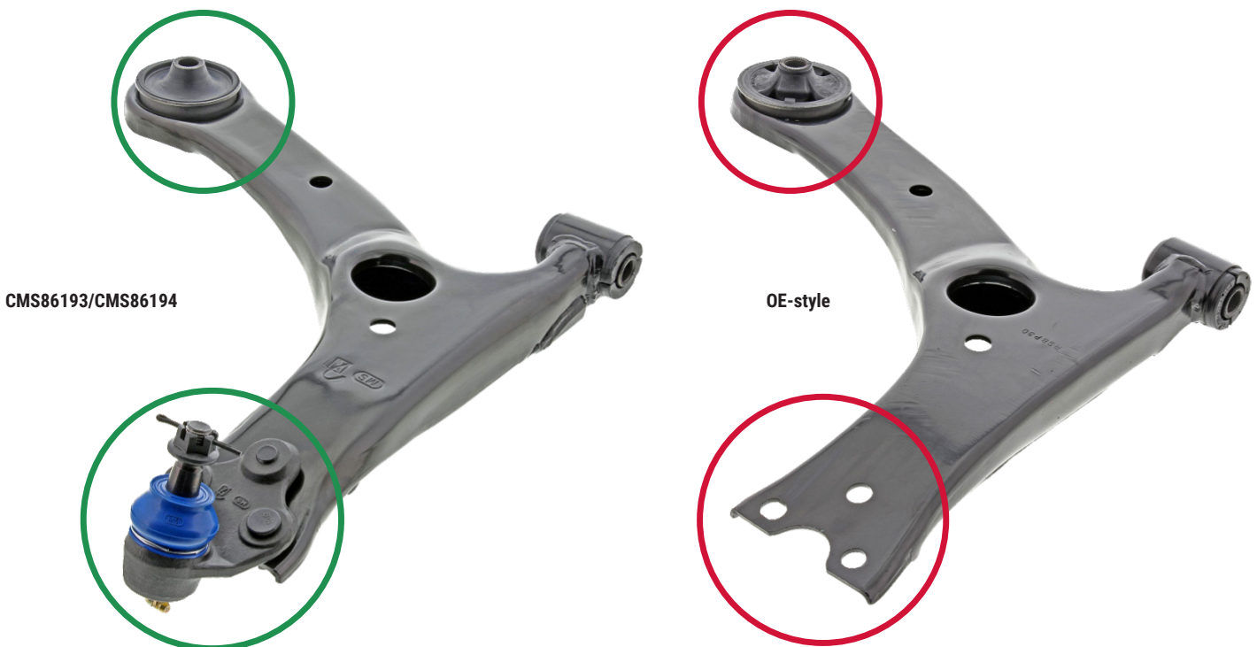
Figure 1. Mevotech Supreme control arm assembly with pre-fitted ball joint and solid bushing (left) vs OE-style control arm assembly (right)
