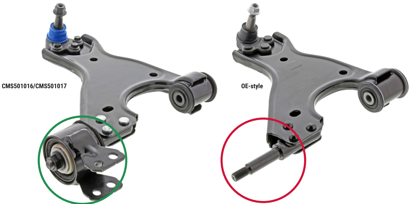
Figure 1. Mevotech Supreme control arm assembly with pre-fitted compliance bushing (left) vs OE-style control arm assembly (right)
