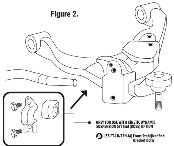
Figure 2. KDSS-equipped vehicles feature a mounting area on the control arm for the stabilizer bar
