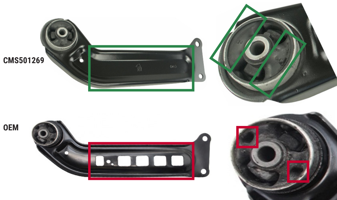
Figure 1. Mevotech Supreme rear trailing arm CMS501269 featuring improved stamping profile with filled-in body and bushing voids (top) vs OEM design (bottom)
