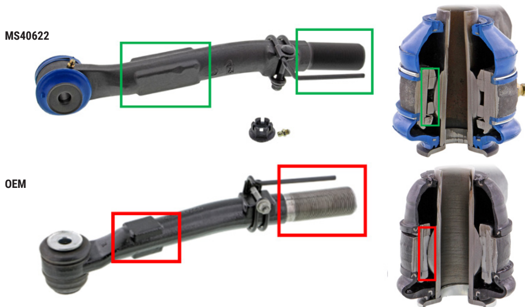
Figure 1. Mevotech Supreme front right outer tie rod end MS40622 with improved forging profile, featuring greaseable, self-lubricating upper and lower sintered bearings, full anti-corrosion coating and included hardware (top) vs OEM with sealed plastic bearing, reduced forging profile and uncoated finish on threaded end (bottom)
