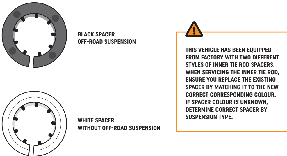
Figure 1: Suspension type and corresponding steering spacer
