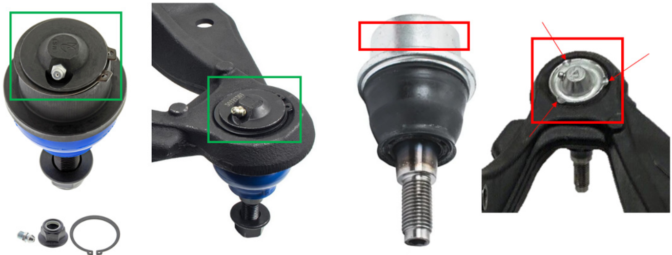
Figure 1. Mevotech Supreme front lower ball joint MS50553 can be secured to the control arm easily via the included circlip (left) vs OEM stake/crimp method (right)
