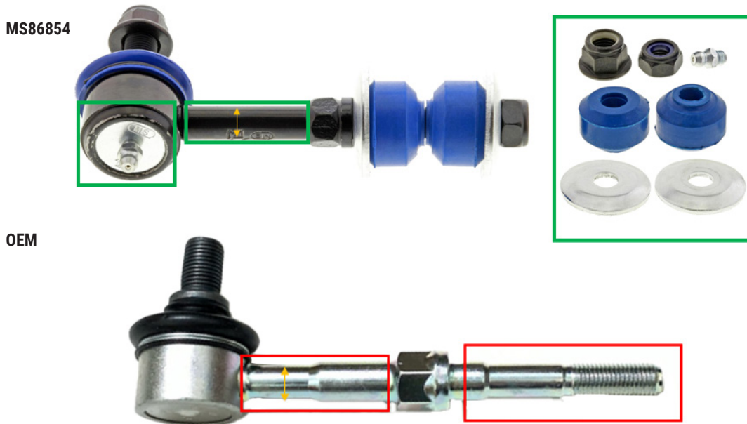
Figure 1. Mevotech Supreme rear stabilizer bar link MS86854 with replacement hardware and bushings, larger diameter connecting rod and greaseable self-lubricating sintered bearings (top) vs the OEM (bottom)
