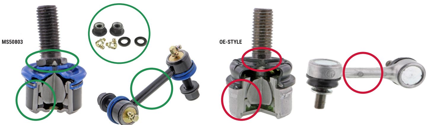
Figure 1. Mevotech Supreme front stabilizer link MS50803 with solid steel design, featuring greaseable self-lubricating upper and lower sintered metal bearings, improved wrench flat for easier install and included hardware (left) vs OEM sealed plastic bearing, reduced wrench flat and lightweight aluminum design (right)
