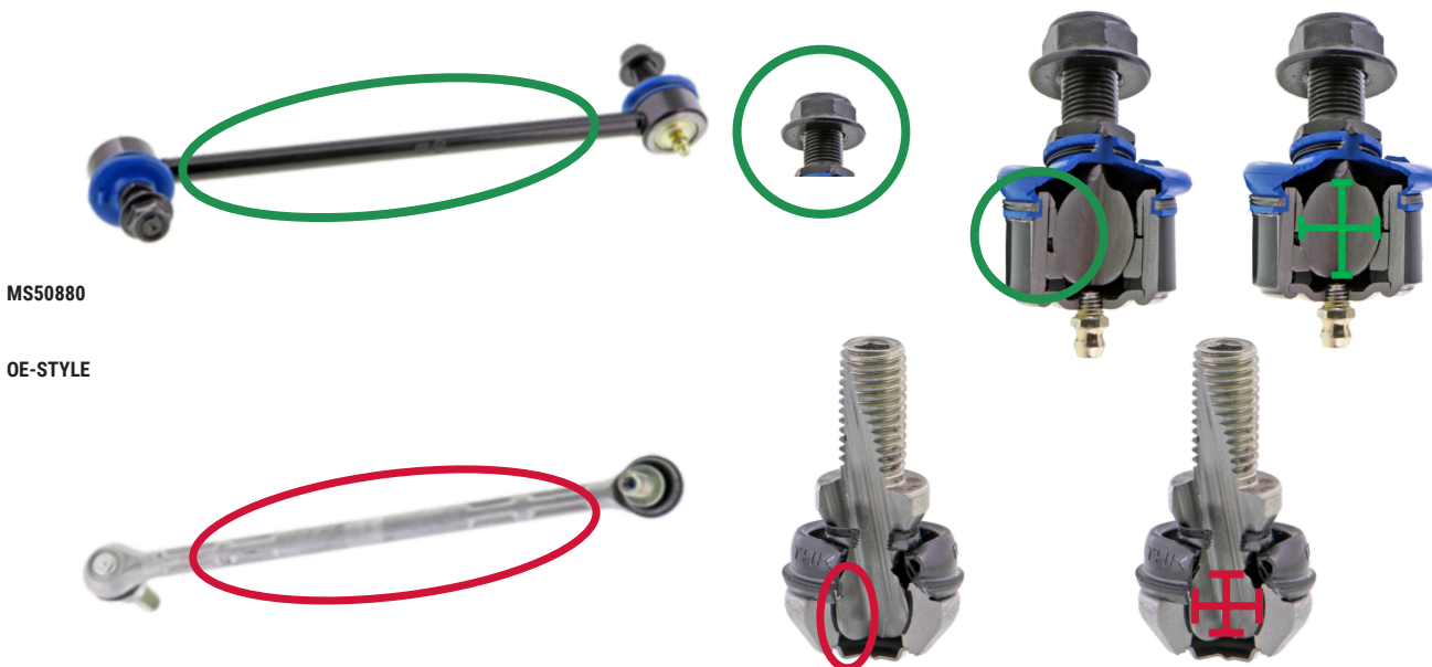
Figure 1. Mevotech Supreme front stabilizer link MS50880 with solid steel construction, featuring greaseable, self-lubricating lower sintered metal bearing, increased ball pin to bearing contact area and included hardware (top) vs OEM with sealed plastic bearing, lightweight aluminum body and reduced ball pin contact area (bottom)
