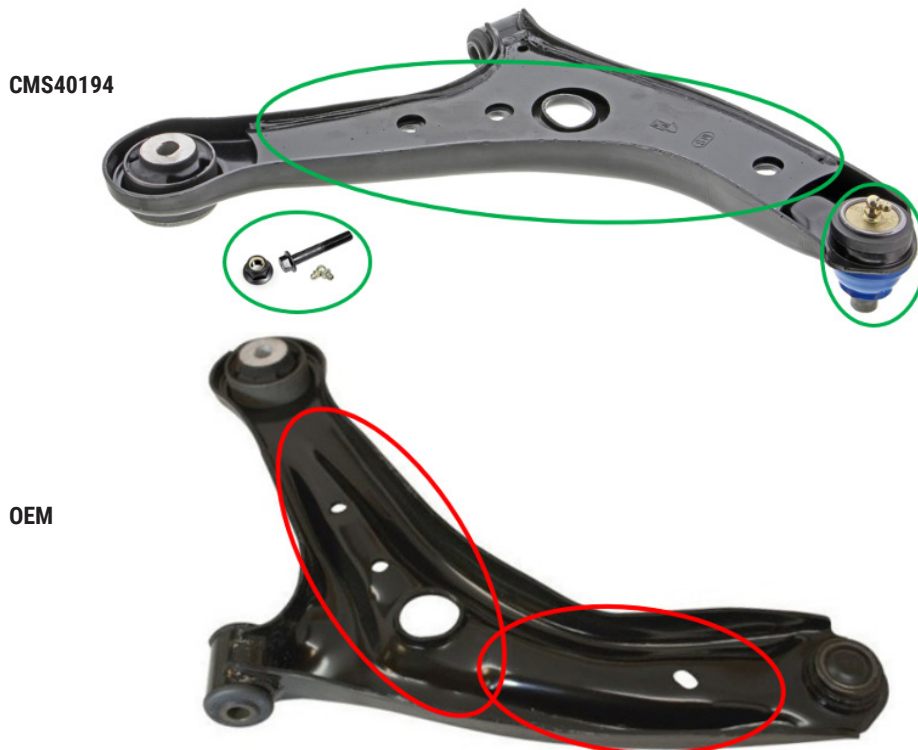
Figure 1. Mevotech Supreme control arm CMS40194 with improved stamping profile, featuring reinforcement plate, greaseable self-lubricated sintered bearing ball joint and included hardware (top) vs OEM design (bottom)
