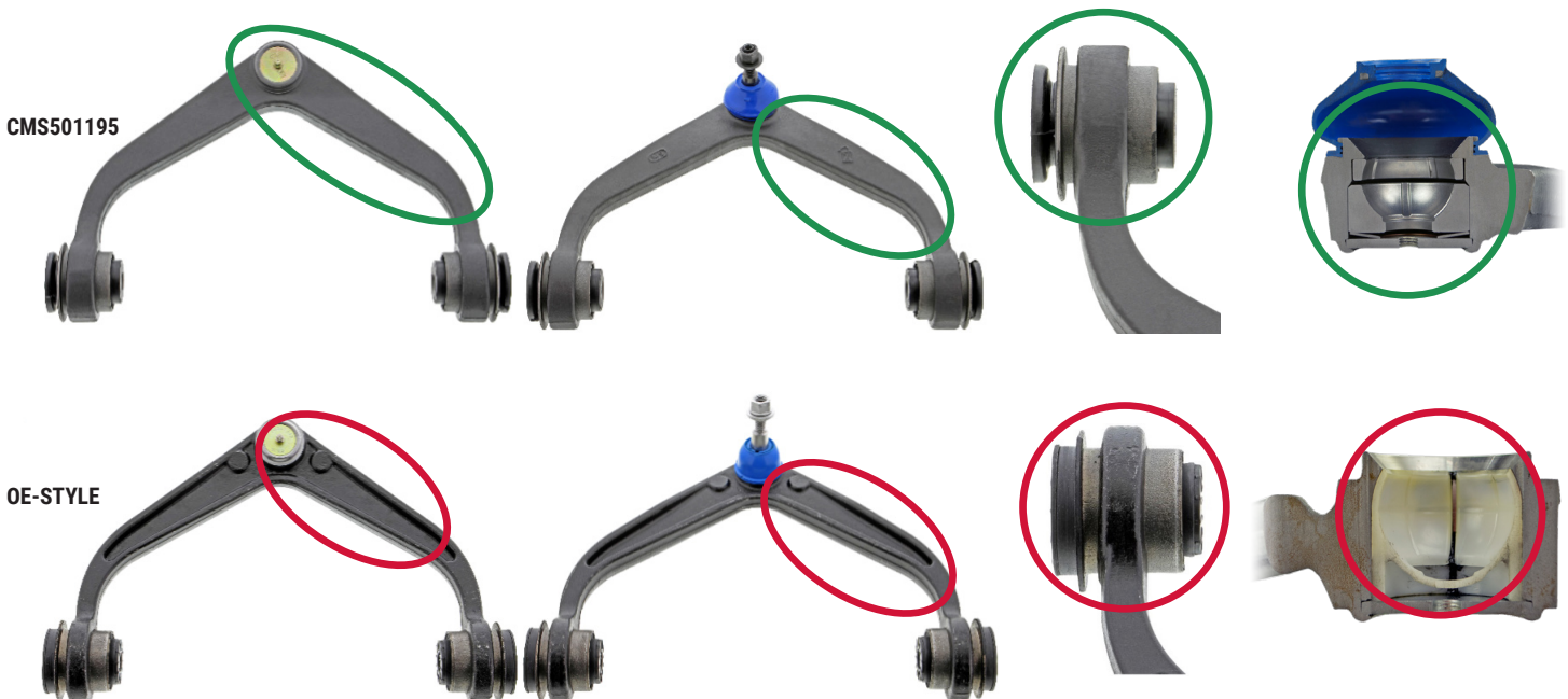
Figure 1. Mevotech Supreme control arm with self-lubricating greaseable sintered metal bearings and improved forging profile (top) vs OE-style control arm (bottom)
