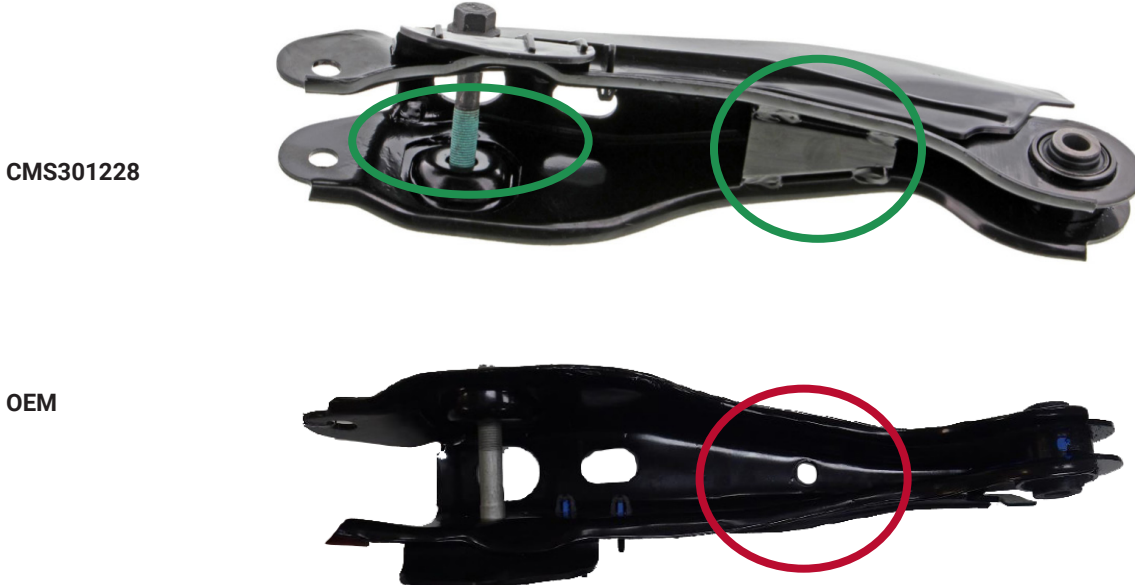
Figure 1. Mevotech Supreme control arm CMS301228 with improved stamping profile, featuring reinforcement plate and included hardware with thread-locking compound (top) vs OEM design (bottom)
