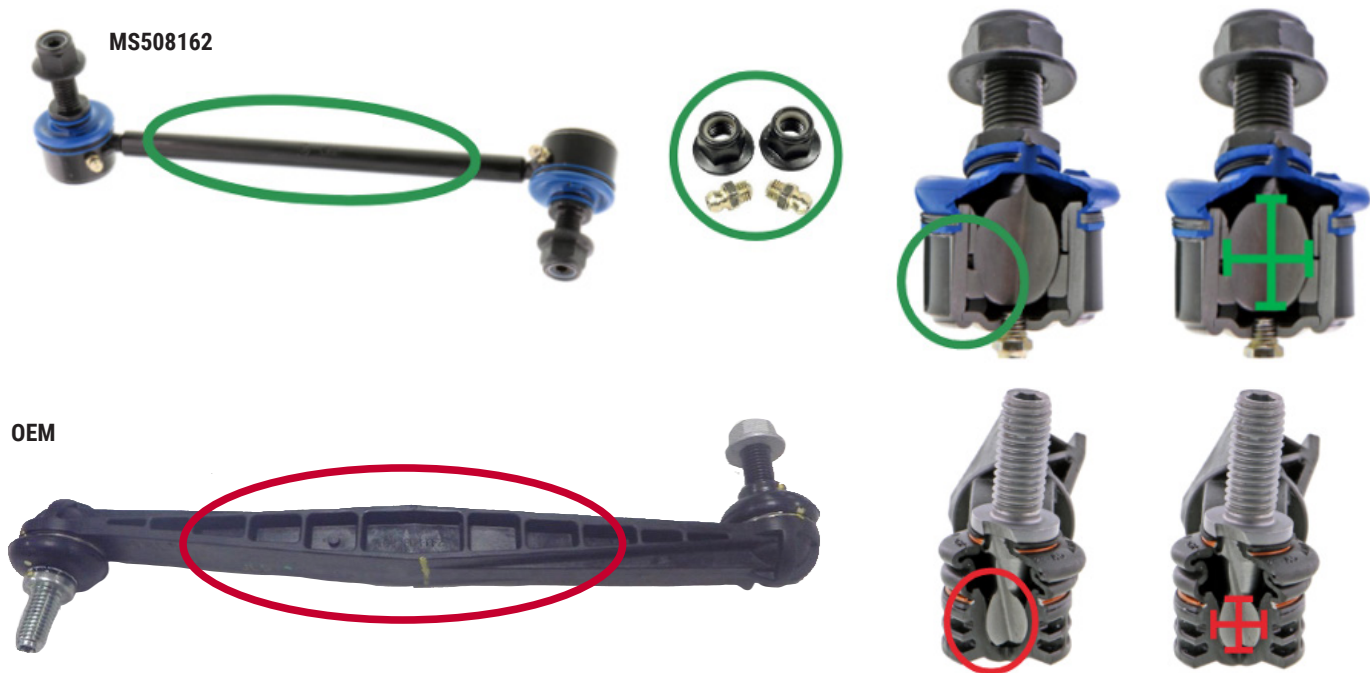
Figure 1. Mevotech Supreme MS508162 with solid steel design, featuring greaseable, self-lubricating upper and lower sintered metal bearings, increased ball pin to bearing contact area and included hardware (top) vs OEM plastic body, sealed plastic housing and reduced ball pin contact area (bottom)
