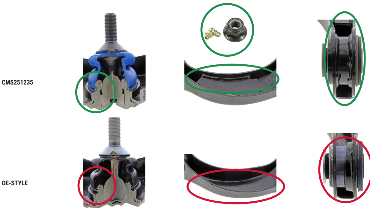
Figure 1. Mevotech Supreme control arm CMS251235 with improved stamped steel profile featuring greaseable self-lubricating sintered upper and lower metal bearings, additional frame and bushing bracing and included hardware (top) vs OEM design and non-serviceable ball joint (bottom)
