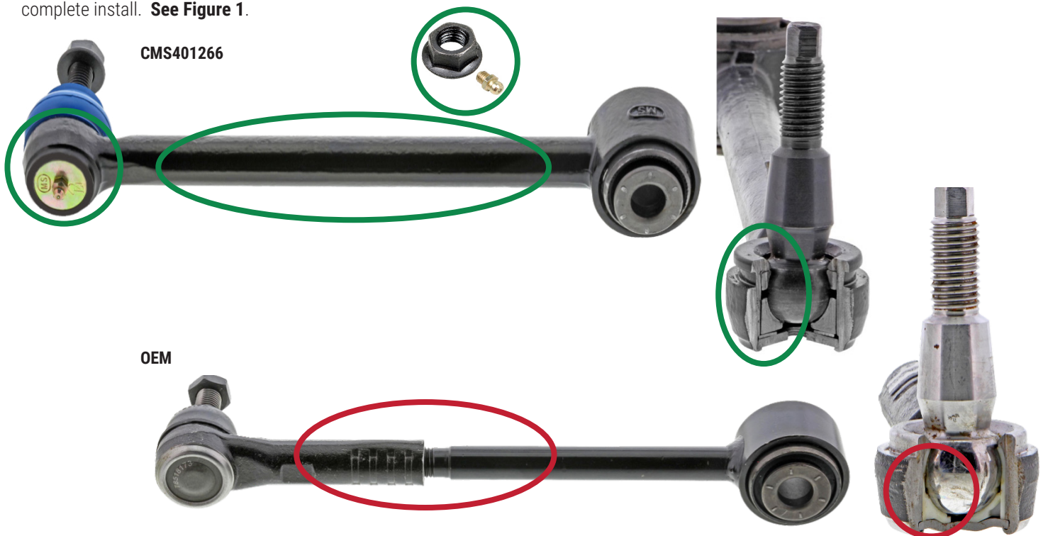
Figure 1. Mevotech Supreme lateral link with greaseable self-lubricating sintered upper and lower metal bearings and improved 1-piece solid forging (top) vs OEM control arm 2-piece design and plastic bearing (bottom)
