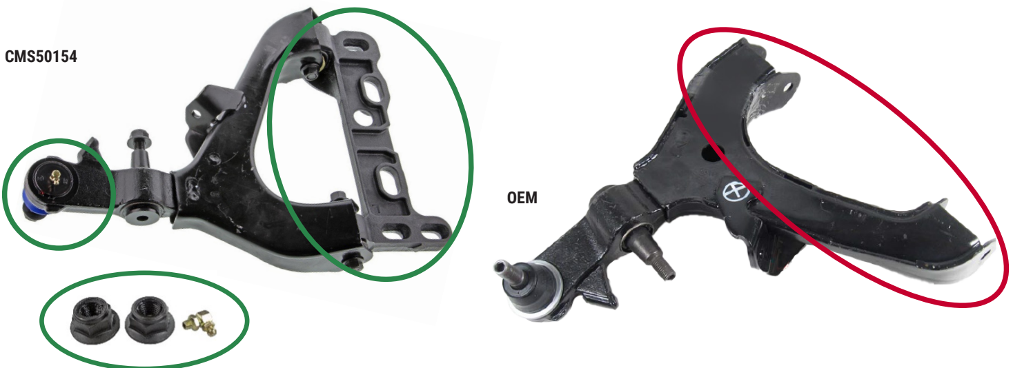
Figure 1. Mevotech Supreme front lower control arm CMS50154 with pre-assembled mounting bracket, greaseable self-lubricating sintered ball joint and hardware (left) vs OEM control arm (right)
