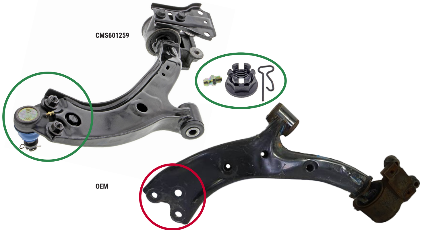
Figure 1. Mevotech Supreme front lower forward control arm CMS601259 pre-fitted ball joint and hardware (top) vs OEM bare control arm (bottom)
