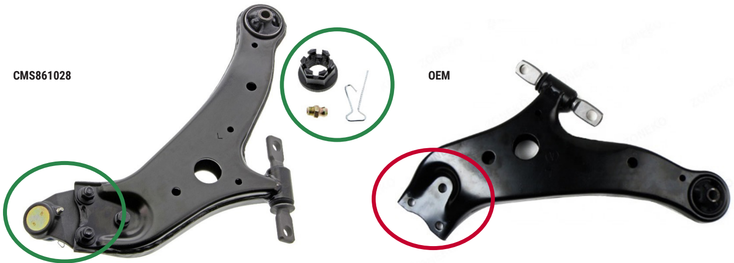
Figure 1. Mevotech Supreme front lower control arm assembly CMS861028 with greaseable self-lubricating sintered bearing ball joint pre-fitted and hardware (left) vs OEM bare control arm (right)
