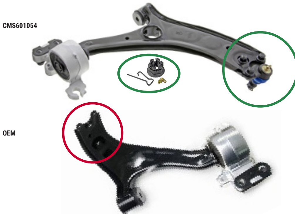
Figure 1. Mevotech Supreme front lower forward control arm assembly CMS601054 with pre-fitted engineered ball joint and hardware (top) vs OEM bare control arm (bottom)
