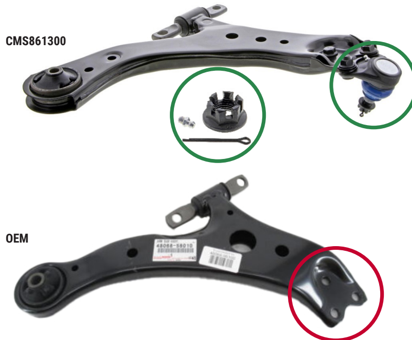
Figure 1. Mevotech Supreme front lower forward control arm assembly CMS861300 with pre-fitted engineered ball joint and hardware (top) vs OEM bare control arm (bottom)
