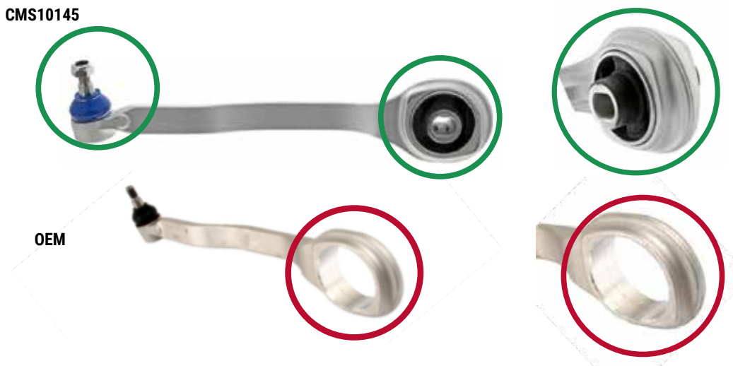
Figure 1. Mevotech Supreme control arm CMS10145 with pre-fitted bushing and fastening hardware (top) vs bare OEM control arm (bottom)
