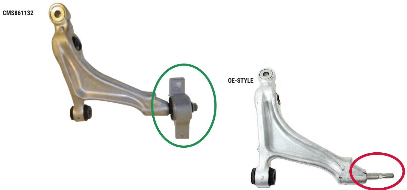
Figure 1. Mevotech Supreme control arm assembly with pre-fitted compliance bushing (top) vs OE-style control arm assembly (bottom)
