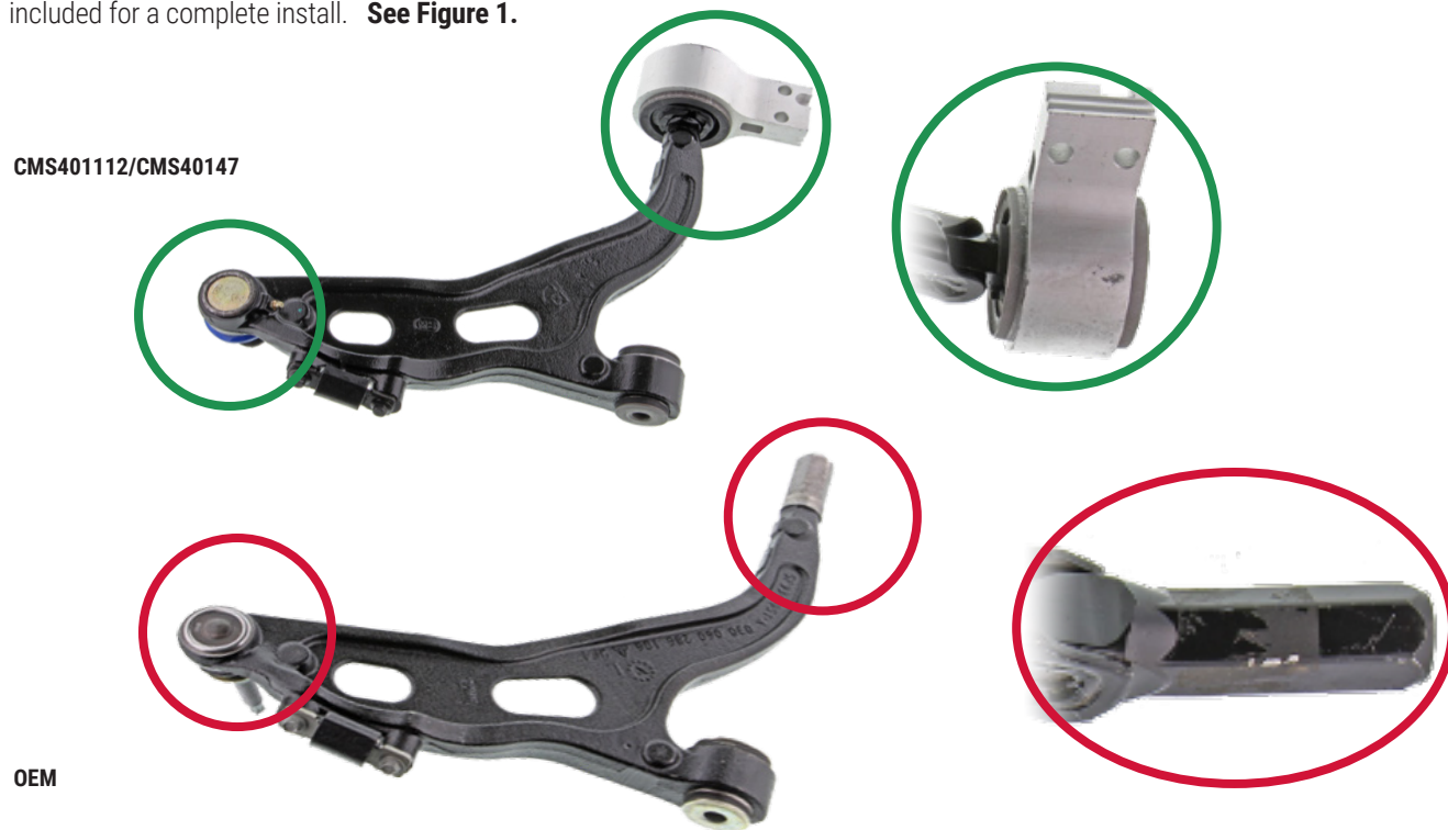
Figure 1. Mevotech Supreme control arm assembly with greasable self-lubricating sintered metal ball joint and pre-fitted compliance bushing (top) vs sealed OEM-style control arm assembly (bottom)
