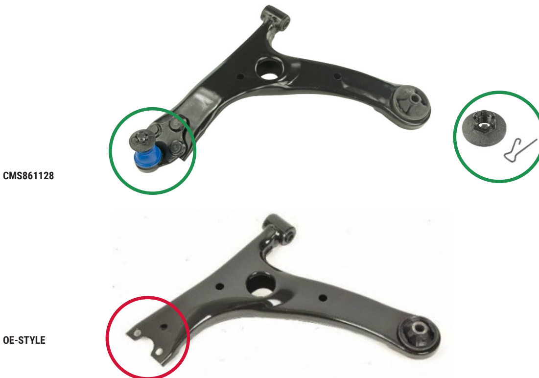
Figure 1. Mevotech Supreme control arm assembly with pre-fitted ball joint and hardware (top) vs OE-style bare control arm (bottom)
