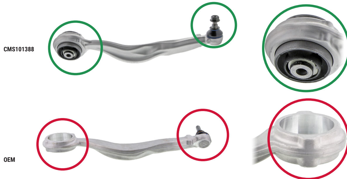
Figure 1. Mevotech Supreme control arm with pre-fitted bushing and hardware (top) vs bare OEM-style control arm (bottom)
